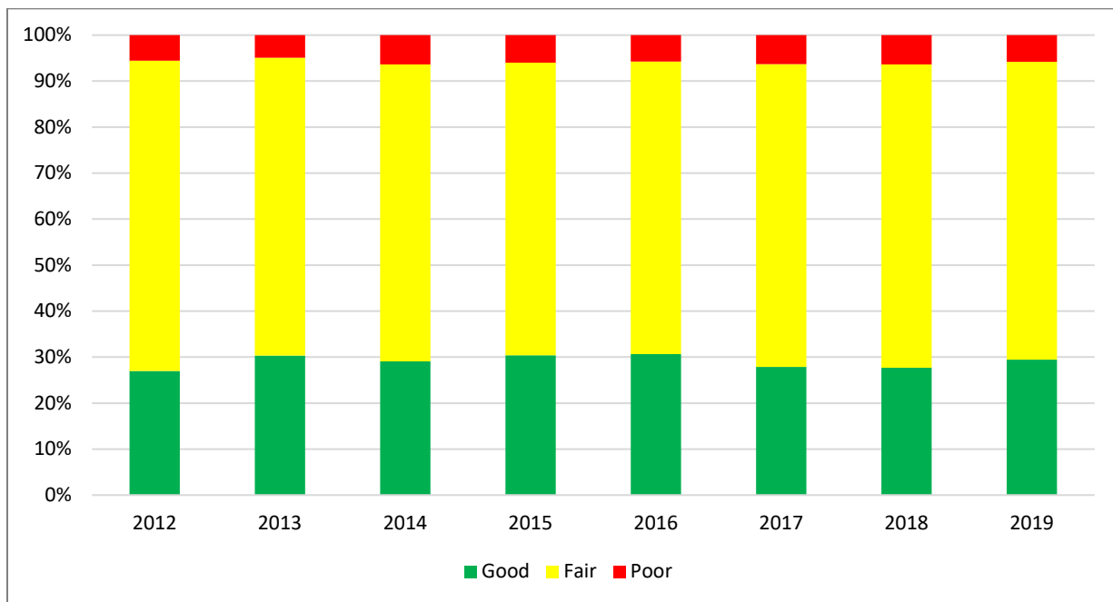
Figure 7-4. Statewide State Highway System Pavement Condition
