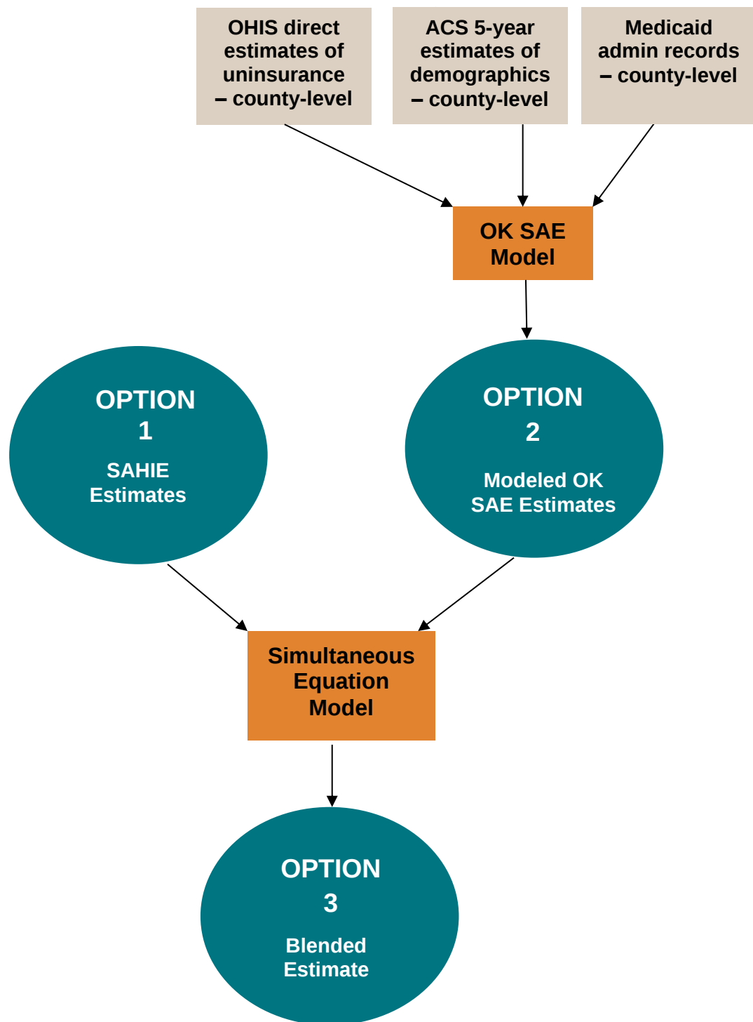
Figure A1. Overview of Options and Small Area Methodology
