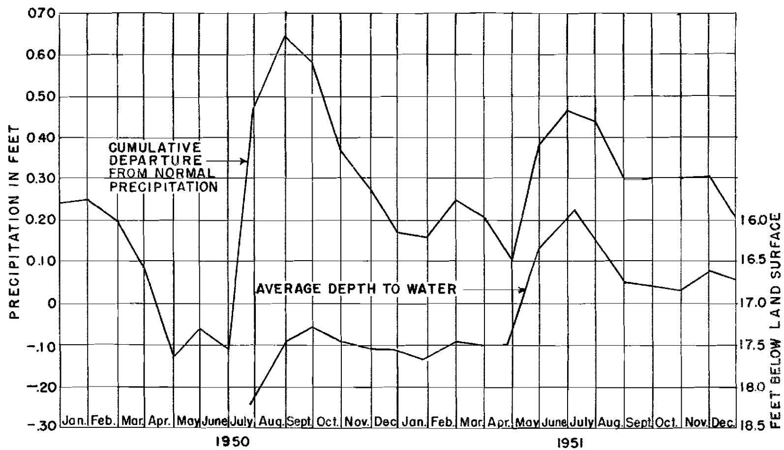
Figure 4.--Fluctuations of average water level in 26 observation wells, and cumulative departure from normal precipitation.
