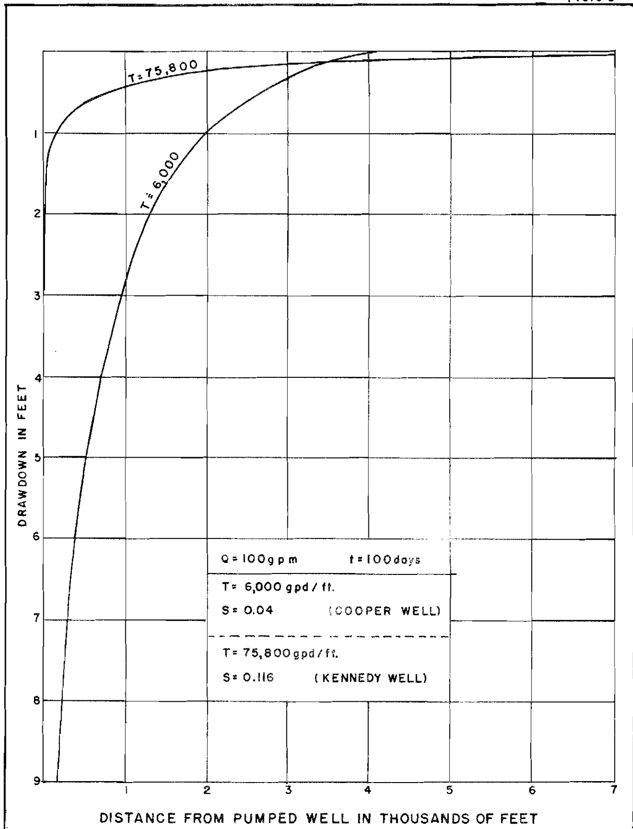
Plate 8.--Theoretical drawdowns of the water level in an infinite aquifer, computed according to the Theis nonequilibrium formula. The Cooper well represents the poorest conditions, and the Kennedy well the best conditions, revealed by the aquifer-performance tests described in this report.
