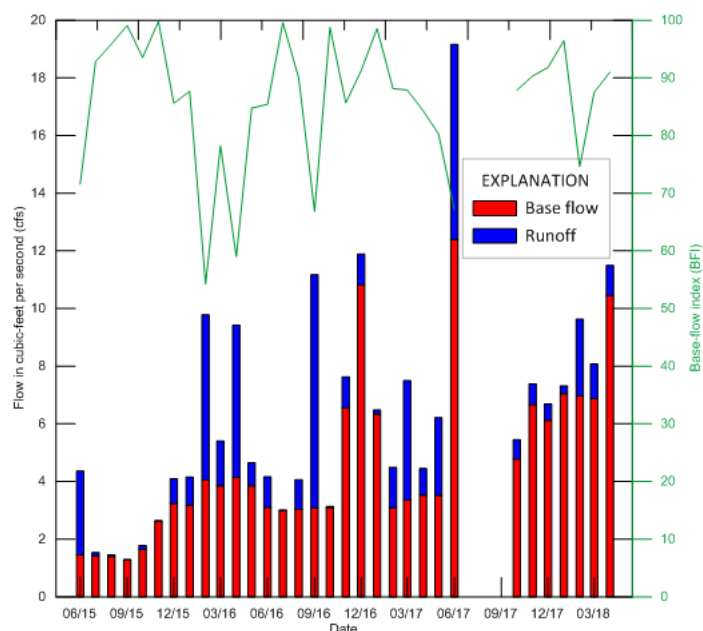
Figure 9. Monthly mean base flow, runoff, and base-flow index for the Trail Creek streamflow gauging station, June 2015-April 2018.
