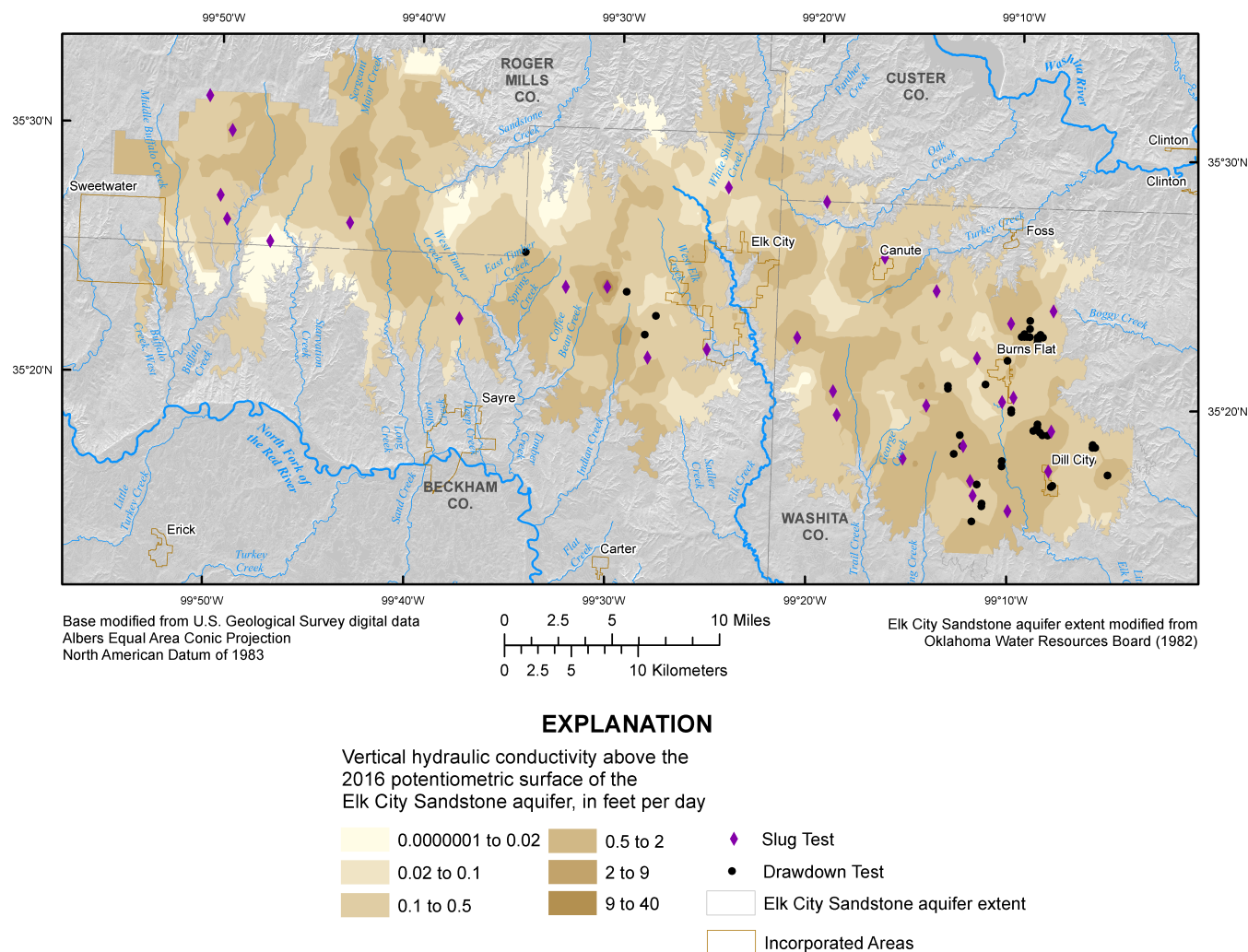
Figure 34. Vertical hydraulic conductivity of the portion of the Elk City Sandstone aquifer above the 2016 potentiometric surface, based on percent-coarse analysis of lithologic descriptions from 1,639 well logs.
