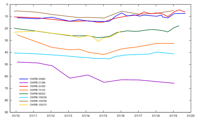
Figure 12. Depth-to-water measurements from Elk City Sandstone wells measured by the OWRB, 2010-19.
