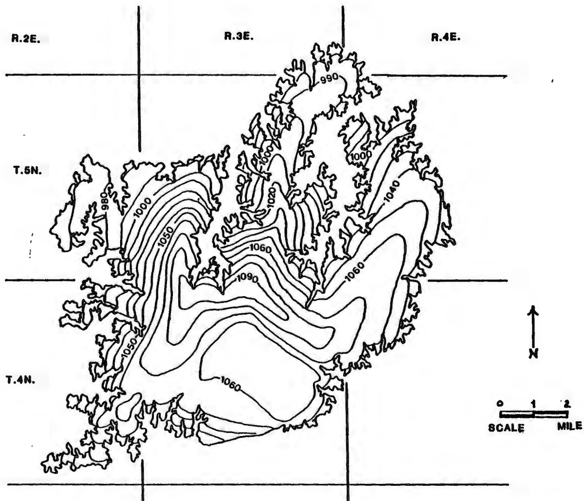
Figure 9. ISOLATED TERRACE DEPOSIT OF THE CANADIAN RIVER OF GARVIN, McCLAIN, AND PONTOTOC COUNTIES, OKLAHOMA. MAY 21 - 22, 1986 WATER TABLE MAP.
