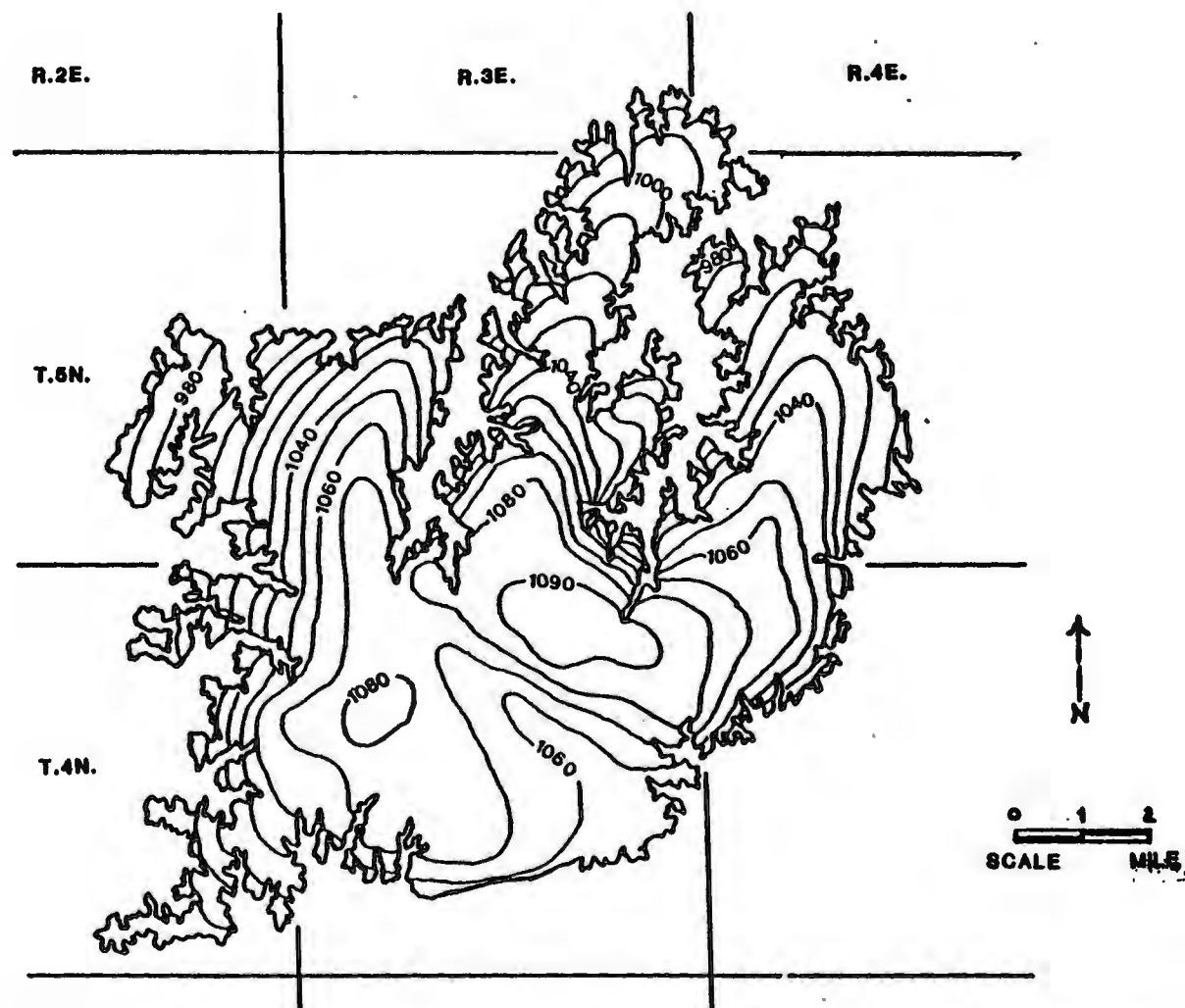
Figure 12, ISOLATED TERRACE DEPOSIT OF THE CANADIAN RIVER OF GARVIN, McCLAIN, AND PONTOTOC COUNTIES, OKLAHOMA. MARCH 5, AND 6, 1986 WATER TABLE MAP.
