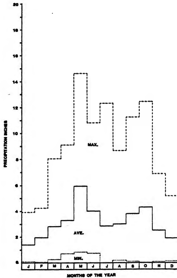
FIGURE 5. MONTHLY PRECIPITATION AT ADA, OKLAHOMA. (1960 - 1986)
