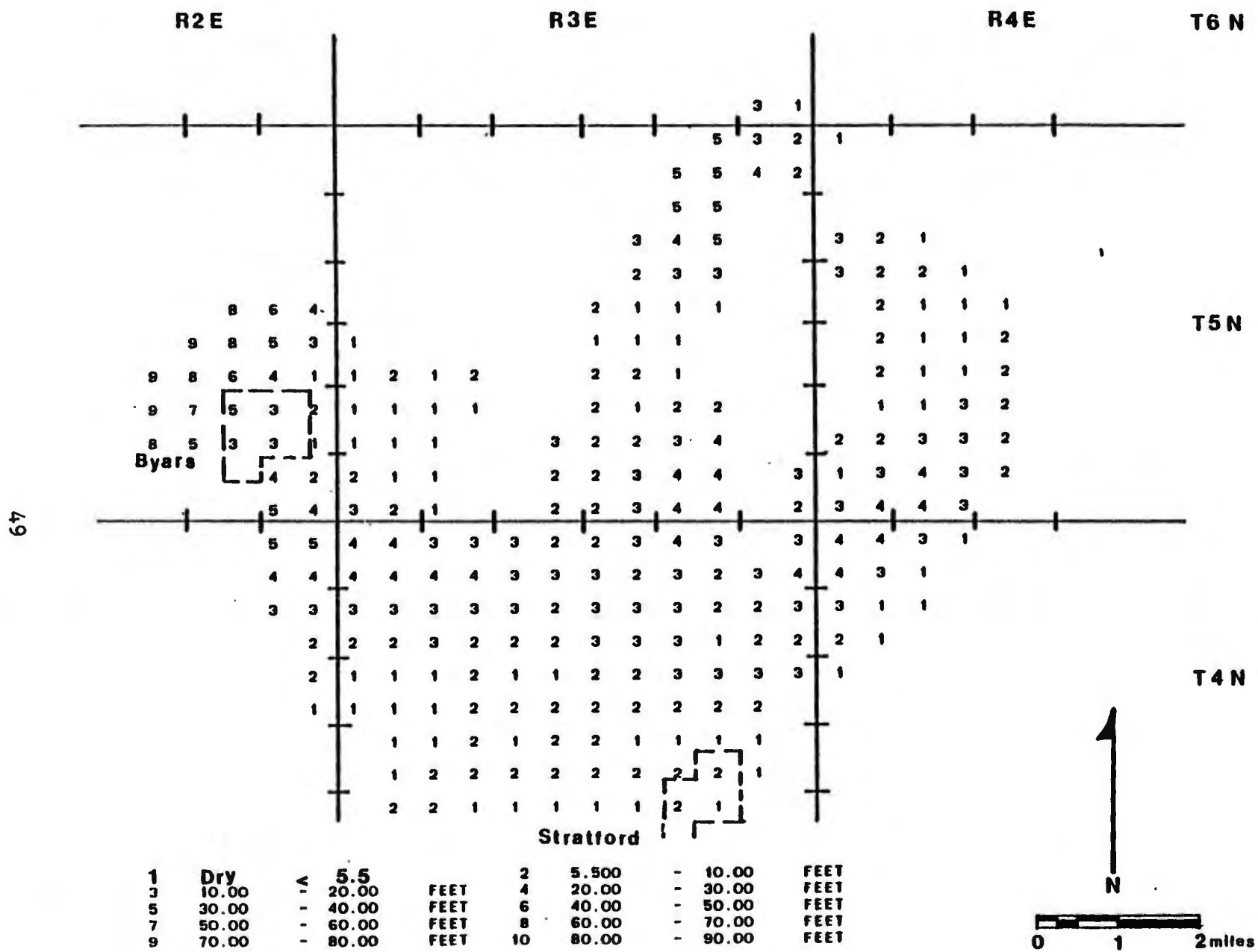
Figure 22. SATURATED THICKNESS ----- 10.00 YEARS
