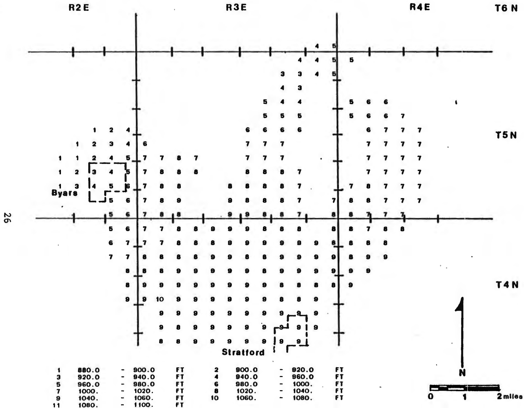
FIGURE 14 Elevation of aquifer bottom
