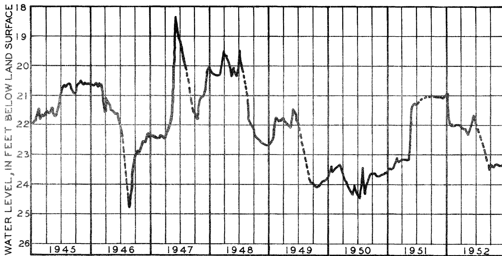
Figure 4.--Water-level fluctuations in well 1S 19W-25.
