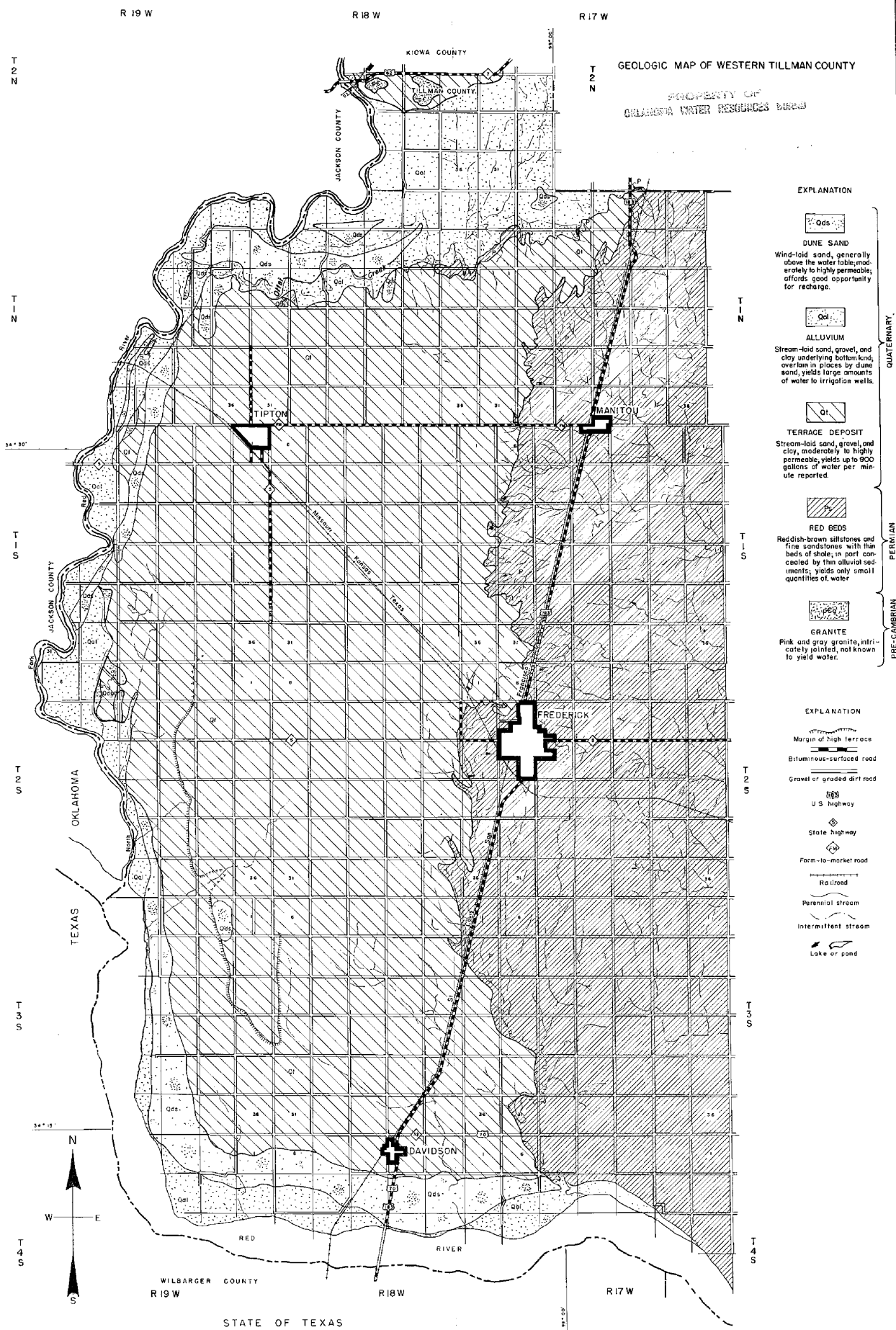
GEOLOGIC MAP OF WESTERN TILLMAN COUNTY, OKLAHOMA
