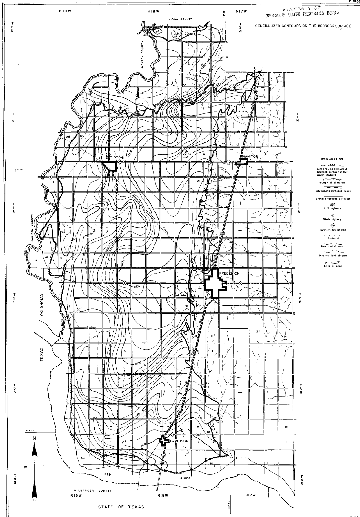
MAP OF WESTERN TILLMAN COUNTY, OKLAHOMA SHOWING GENERALIZED CONTOURS ON THE BEDROCK SURFACE
